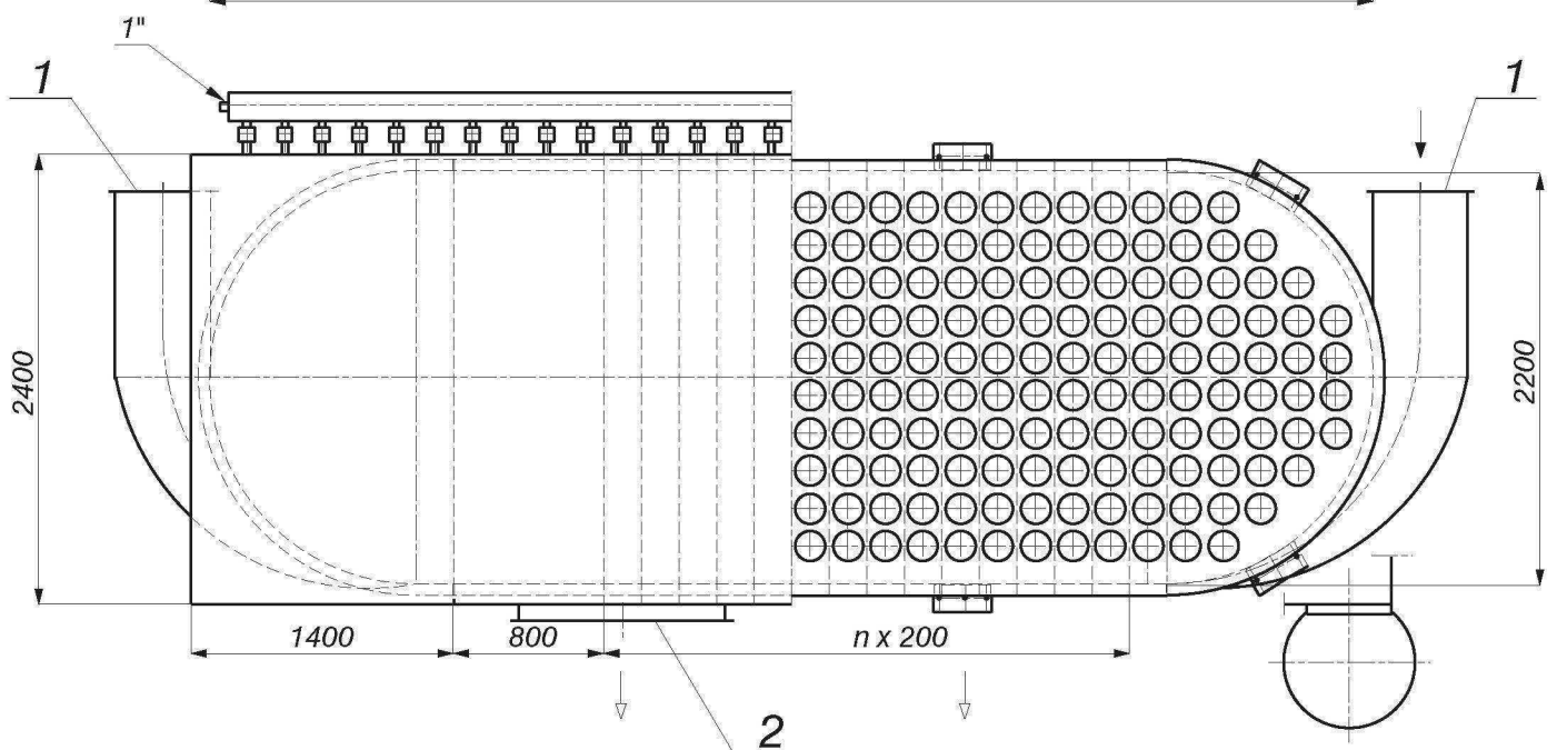
Pulse Jet Filter type DF (136 - 276) - with two rotary rakes
