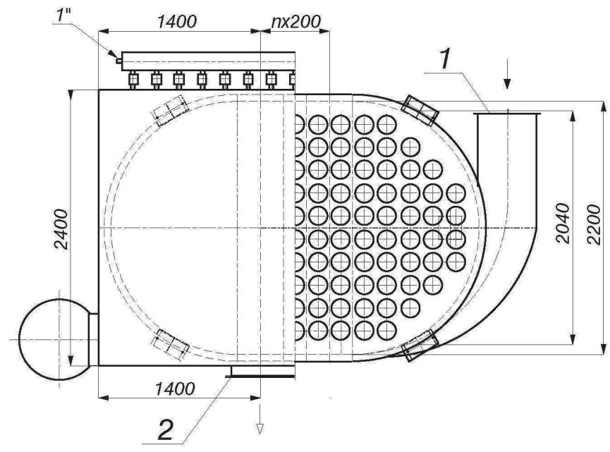
Pulse Jet Filter type DF - with one rotary rake
