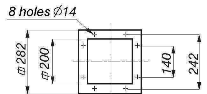
Rotary valve flange 3
